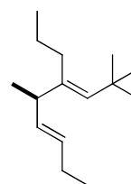
(R,3E,6E)-2,2,5-trimethyl-4-propylnona-3,6-diene
